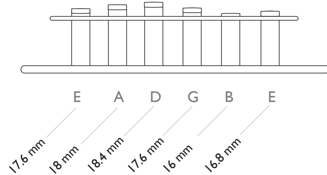
SINGLE COIL 54 VINTAGE STAGGER SIDE PROFILE
