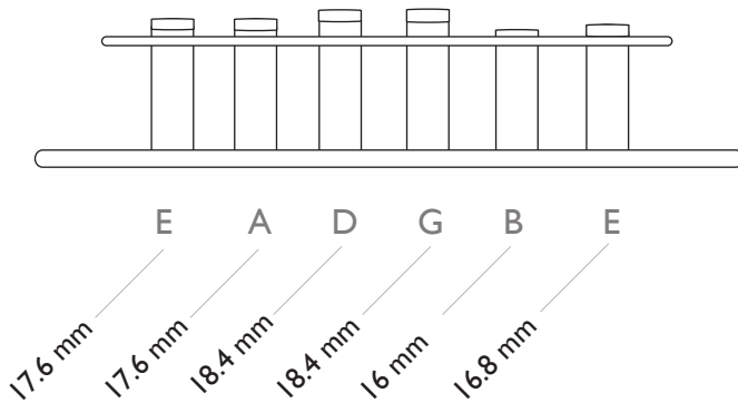
SINGLE COIL 56 VINTAGE STAGGER SIDE PROFILE
