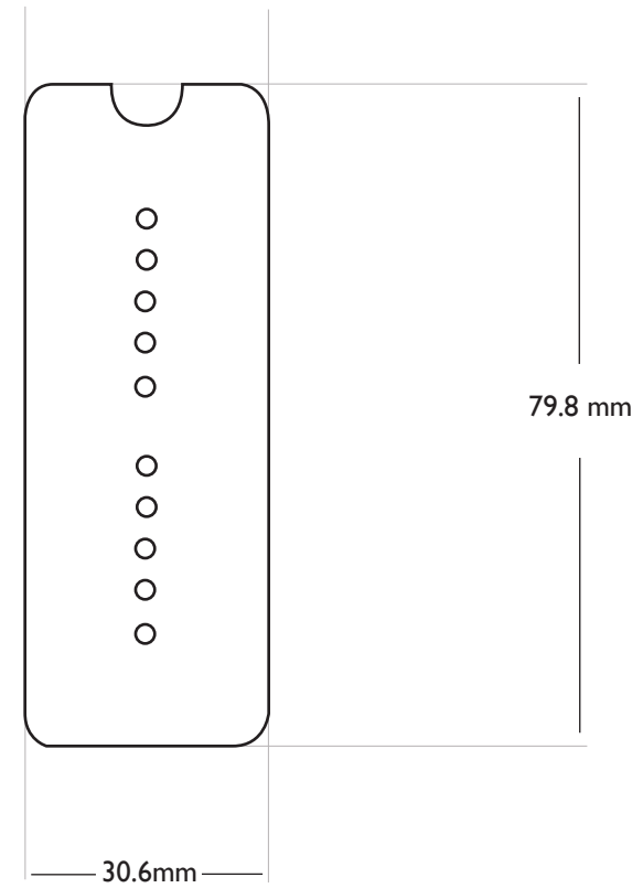
BKP90 BASEPLATE
