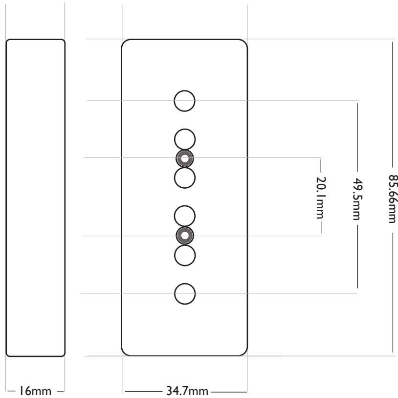
BKP90 COVER
