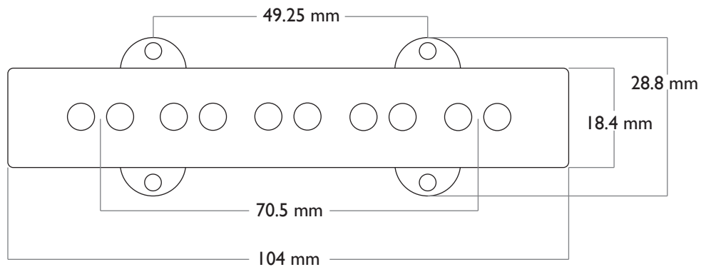
J-BASS 5 STRING BRIDGE
