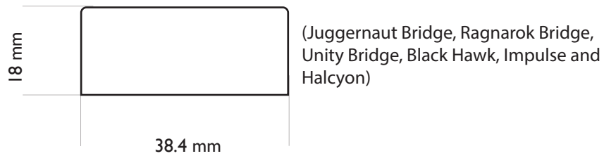
8 STRING SOAPBAR WIDTH & HEIGHT DIMENSIONS (BRIDGE & NECK)
