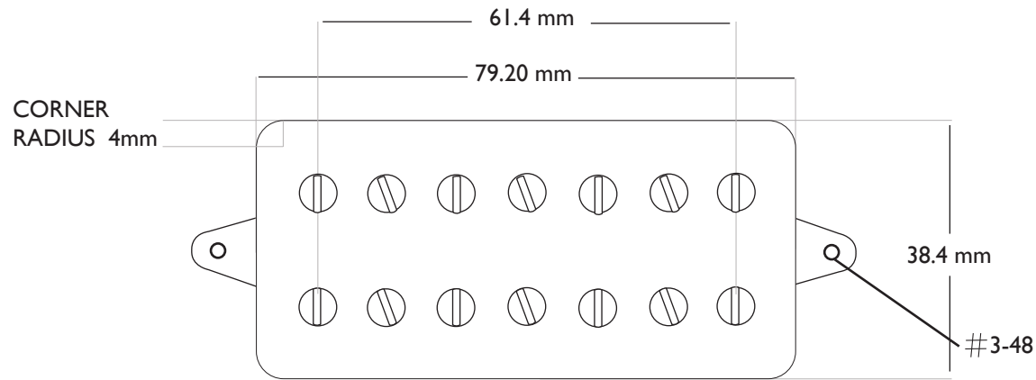
7 STRING COVER DIMENSIONS
