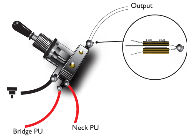
3 Way Toggle Switch
