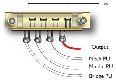
5 Way Pickup Selector
