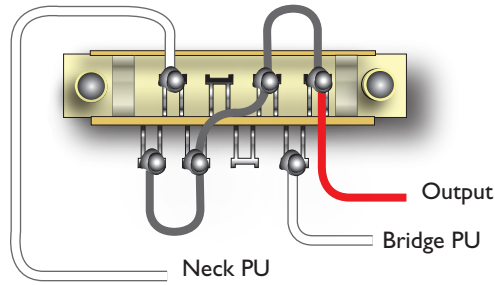
3 Way Pickup Selector
