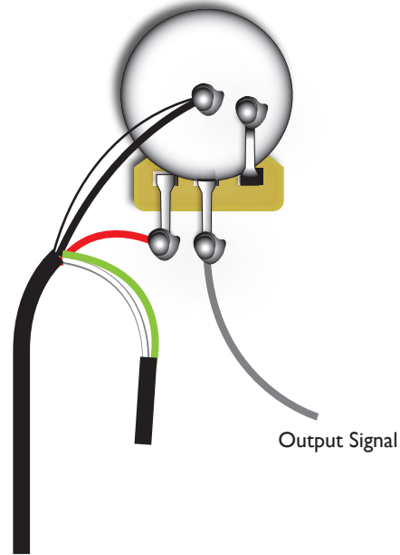
4 Conductor Wiring
