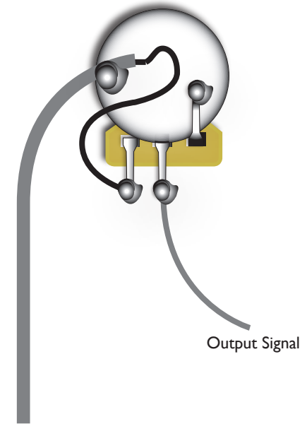
Braided 2 Conductor Wiring
