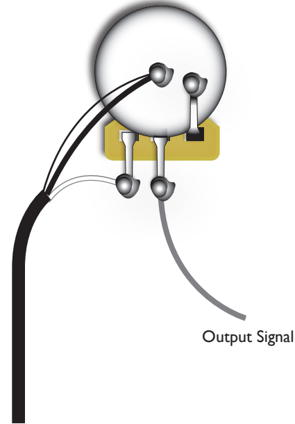
2 Conductor + Screen Wiring
